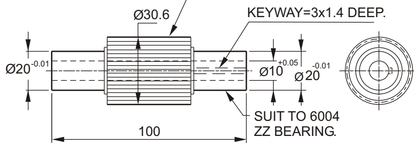
PULLEY.
