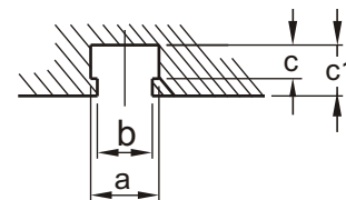
Detail X4:1
